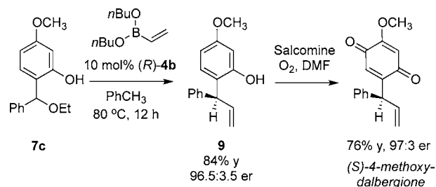
Scheme 3. Synthesis of ( S )-4-Methoxydalbergione
